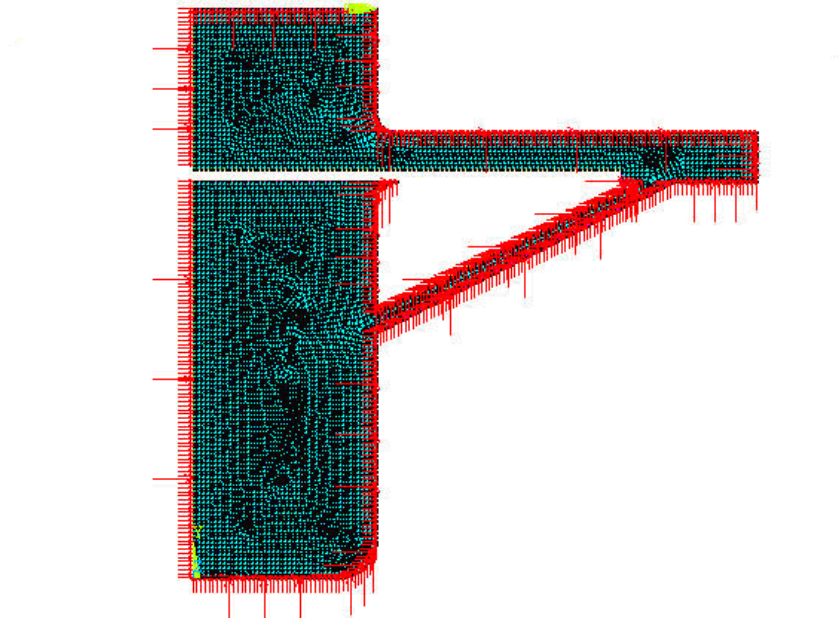
Fig.5 Boundary and loading conditions of the hydro forming deep drawing process
