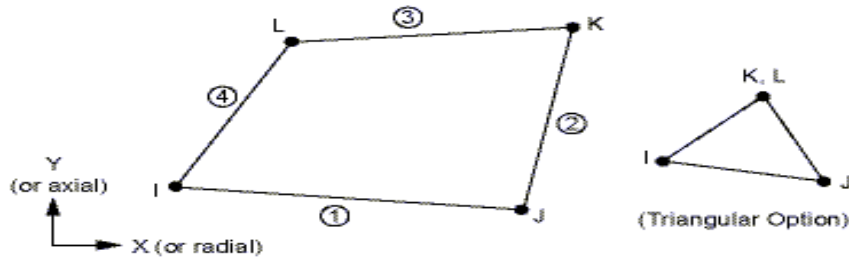
Fig.2 Geometry of FLUID 141 Element
