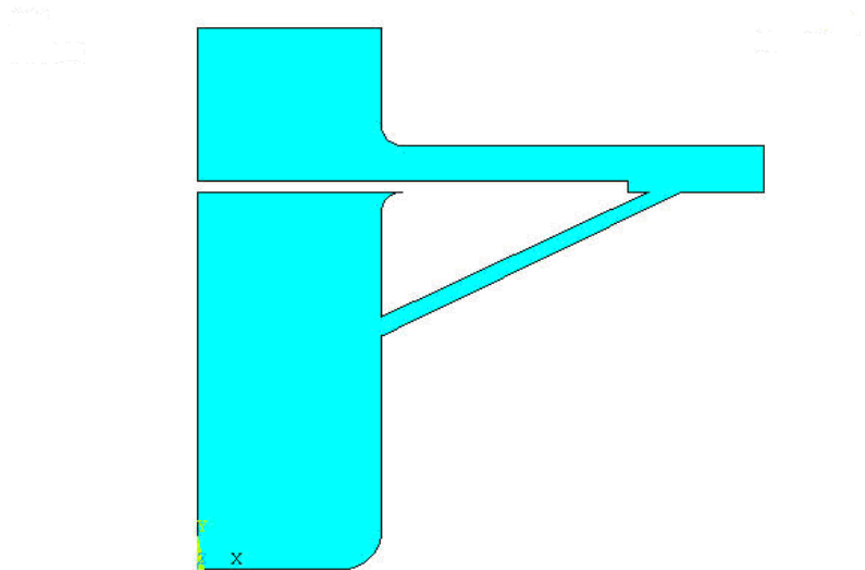
Fig.3 Geometric fluid model ( axisymmetric ) of the hydro forming deep drawing process
