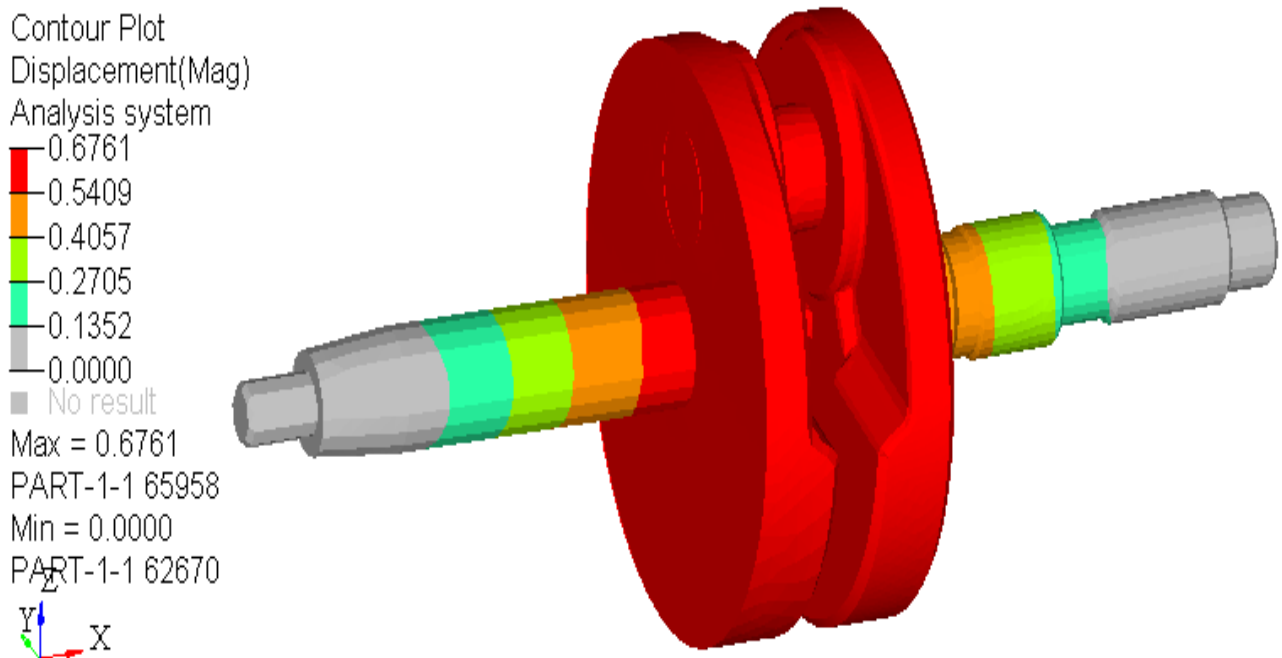
Fig.3. Displacement plot of benchmark crankshaft
