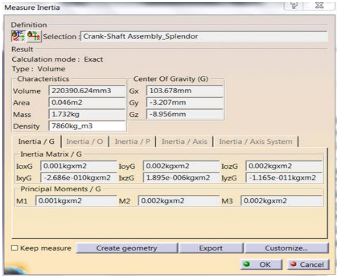
Fig. 5 Mass of benchmark geometry
