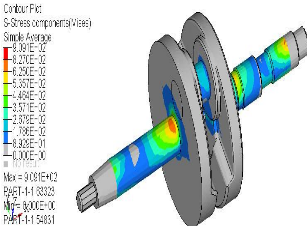
Fig. 4Von mises stress plot of benchmark crankshaft
