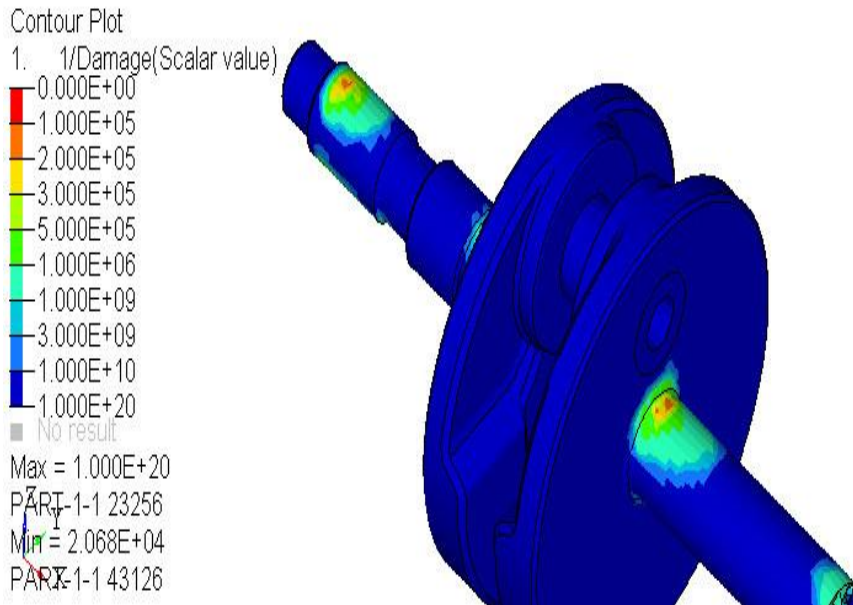
Fig. 11 Fatigue life plot of modified crankshaft
