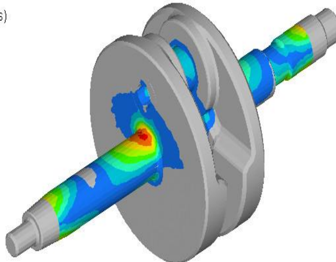
Fig. 9 Von mises stress plot of modified crankshaft
