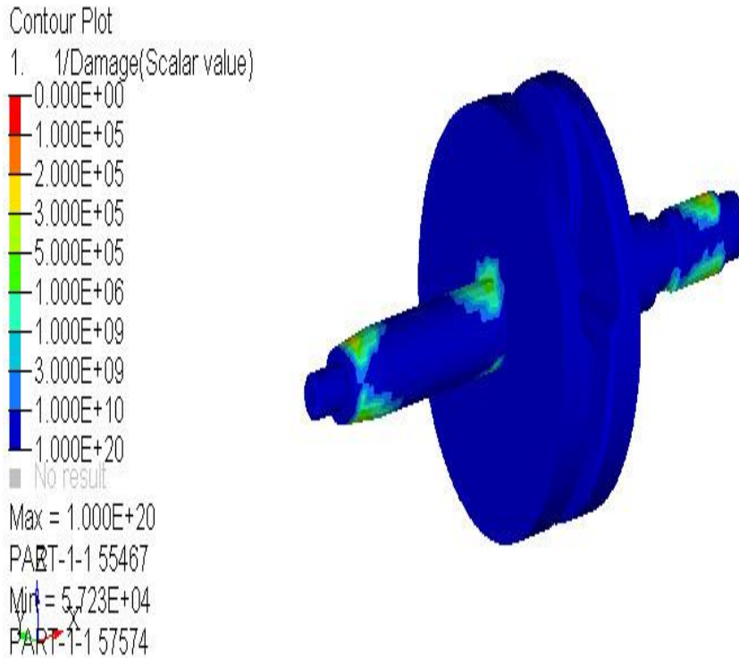
Fig. 7Fatigue life plot of benchmark crankshaft
