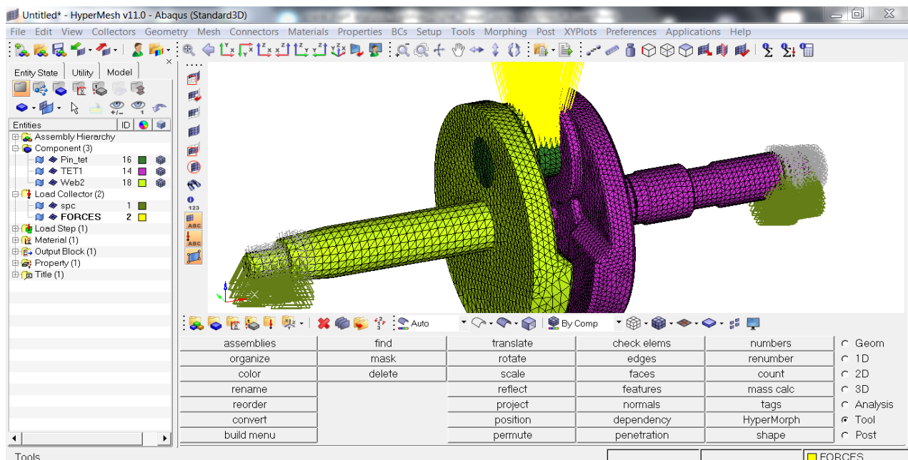
Fig.2.Loads and boundary conditions
