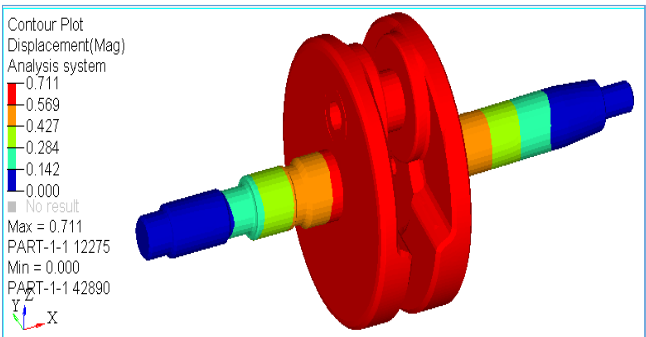
Fig. 8Displacement plot of modified crankshaft
