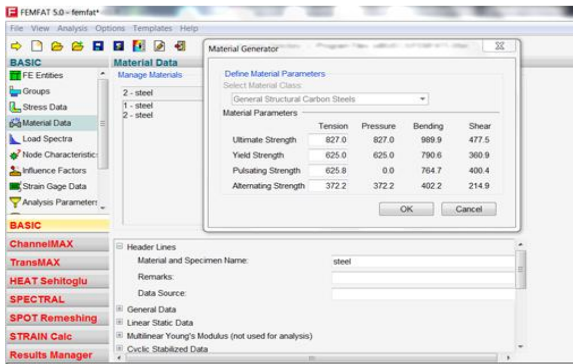
Fig. 6 Inputs to FEMFAT 5.0
