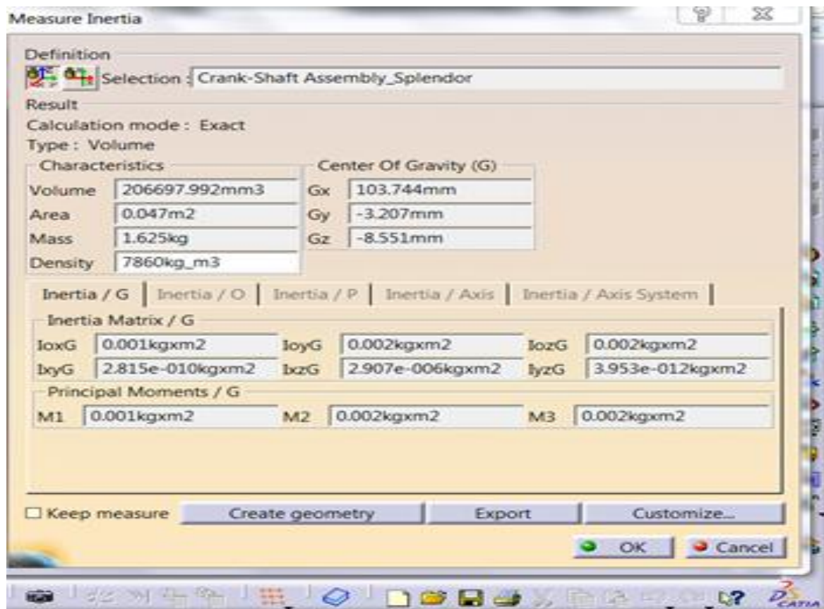
Fig. 10 Mass of modified crankshaft
