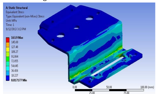
Existing Von-mises Stress Plot
