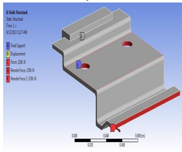
Comparison of Existing & New Design 10. New Boundary Condition Plot
