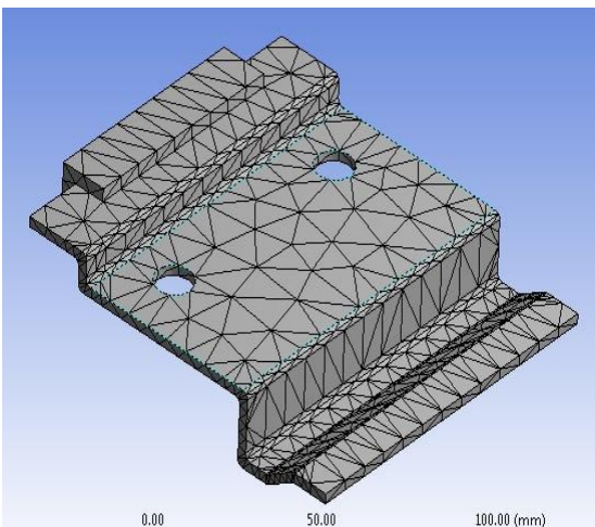
New Design 9. New Meshed Model
