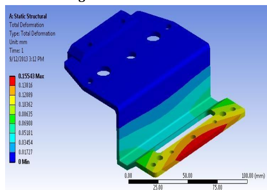
Existing Total Deformation Plot
