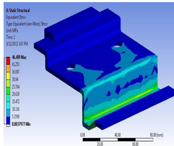
New Boundary Condition Plot 12. New Von-mises Stress Plot
