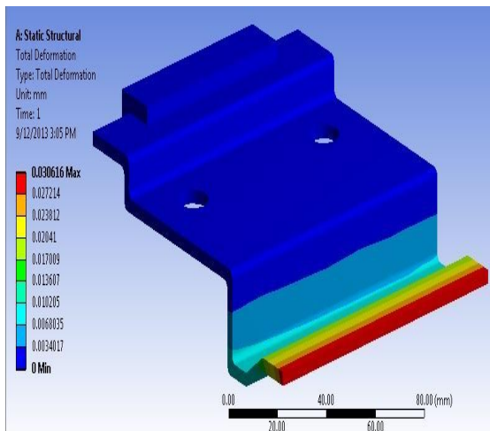
New Meshed Model 11. New Total Deformation Plot
