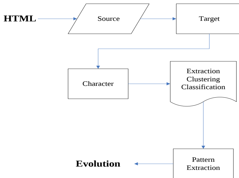
Figure 2: Architecture of Web Text Mining
