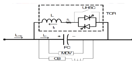
Figure1. Practical module of TCSC
