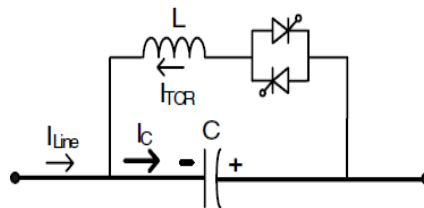
Figure4. Capacitive Boost Mode
