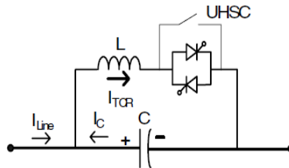
Figure2. Thyristor Bypassed Mode
