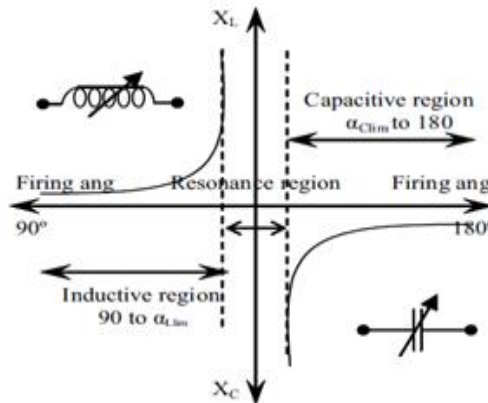
Figure6 Reactance characteristics curve
