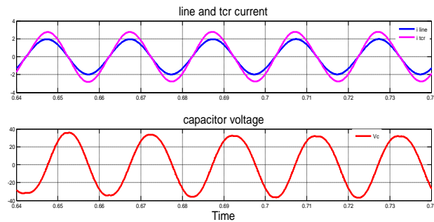
Figure 14 waveform of line current TCR current and capacitor voltage for 0^\circ For purely inductive the power flow is around 591 W which is reduced as above. FOR 25^\circ FIRING ANGLE (INDUCTIVE MODE)
