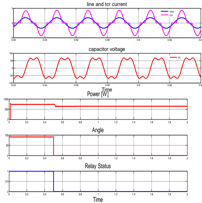
Figure 13 waveform of Power, Angle and Relay status for 0^\circ
