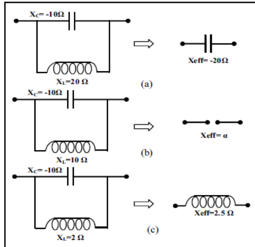
Figure7. Basic characteristics of TCSC
