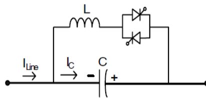
Figure3. Thyristor Blocked Mode
