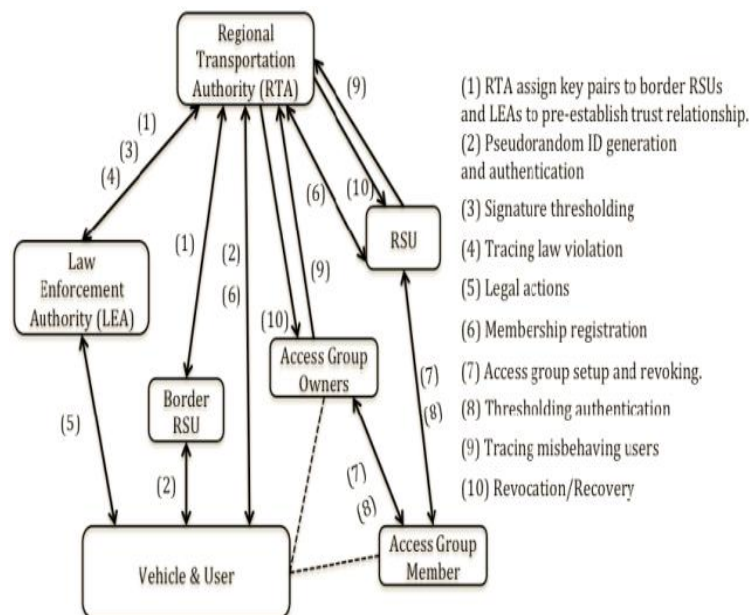
Fig -5: Interactions of the IDbased Security System. [5]
