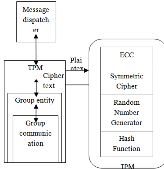
Fig -4: Trust Grouping Framework and TPM architecture.
