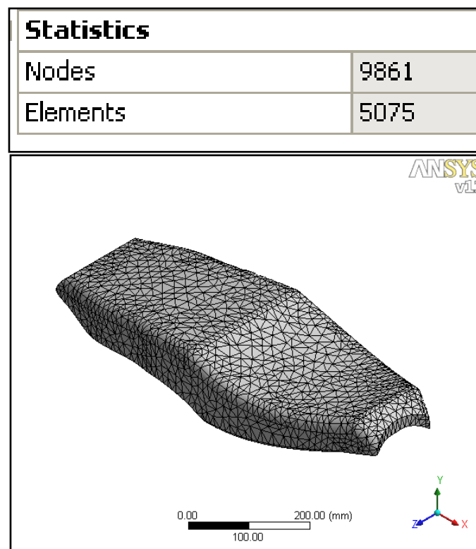
Figure 5.3 Tetrahedron Type of Regular Meshing of Seat A
