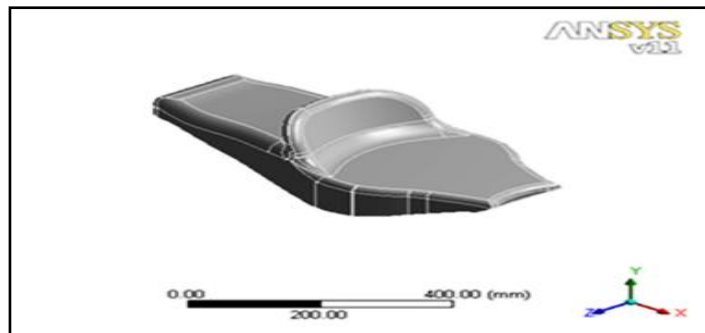
Figure 5.2 Model of Seat B (with lumbar support)
