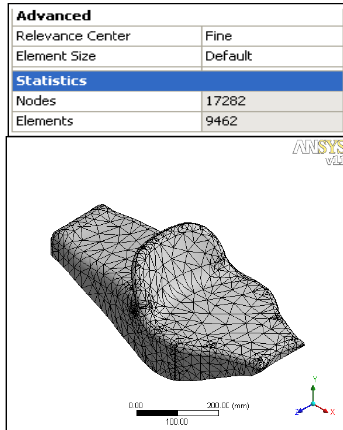
Figure 5.4 Tetrahedron Type of Regular Meshing of Seat B
