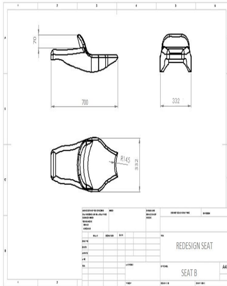
Figure 3.2 Two dimensional design of seat B
