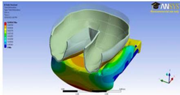
Figure 2.1. Two-layer, rigid steel and flexible skin (neoprene) indenter model in ANSYS V13
