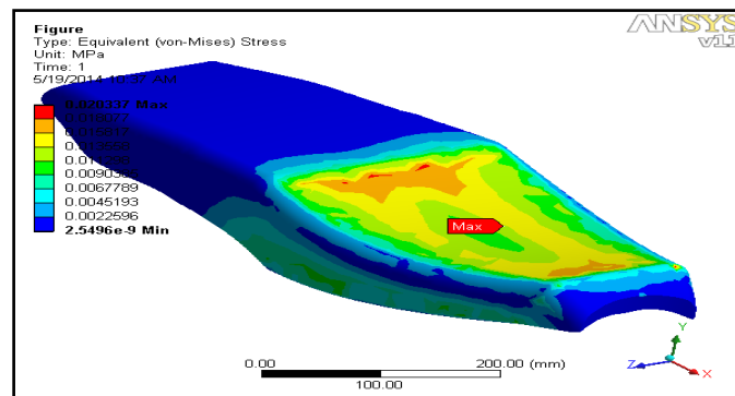
Figure6.1.2 Equivalent / Resultant Stress Induced in seat
