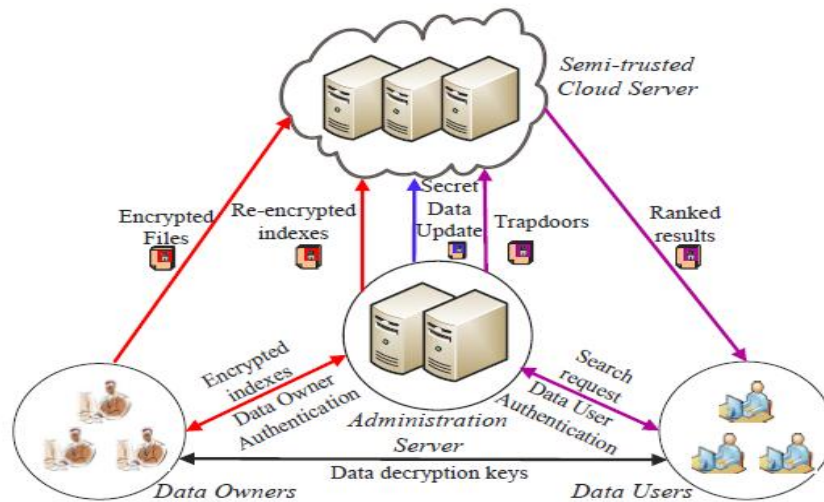
Figure 2: Architecture of multi-keyword synonym query over encrypted cloud data.
