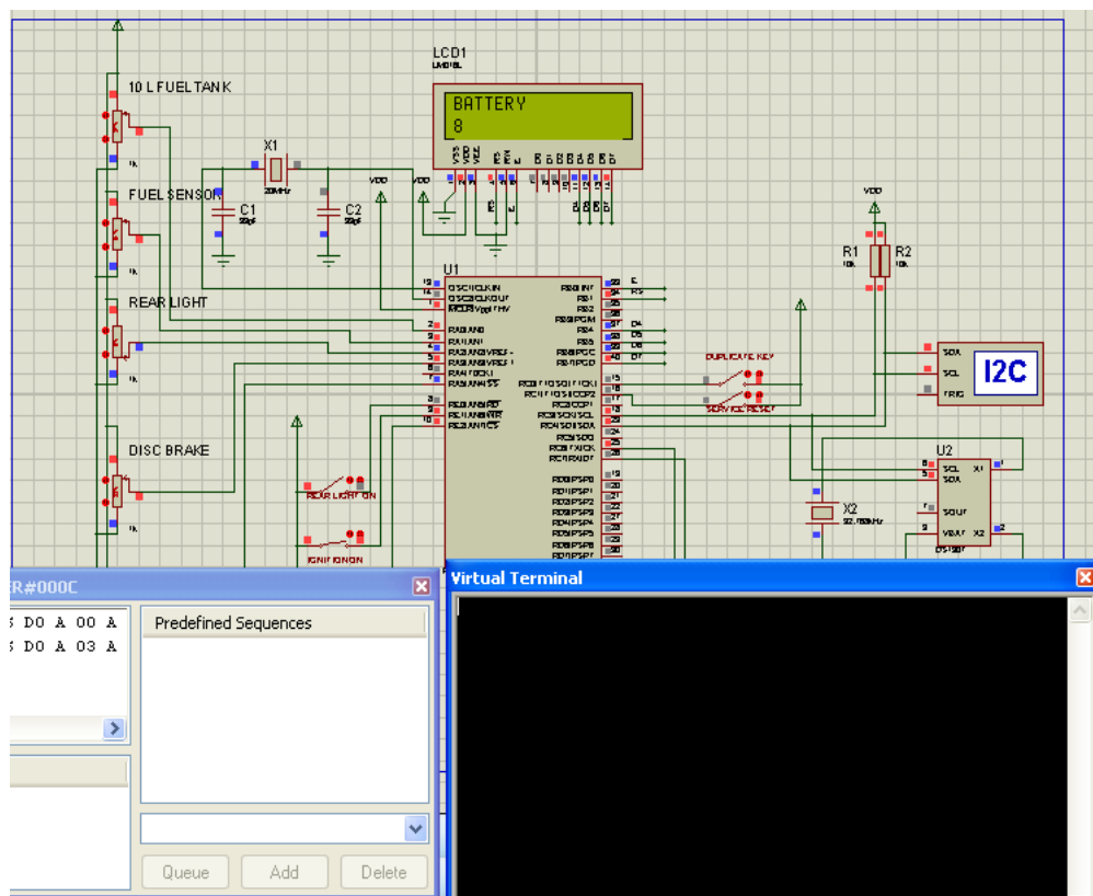
Figure 3: Simulated Output
