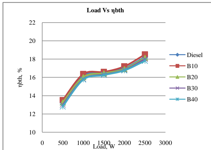
Load Vs Brake Thermal Efficiency
