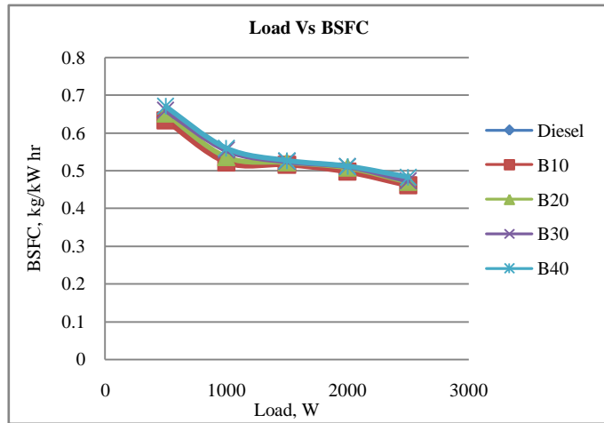
Load Vs Brake specific fuel consumption
