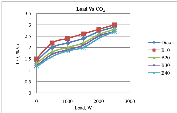
Load Vs Carbon dioxide
