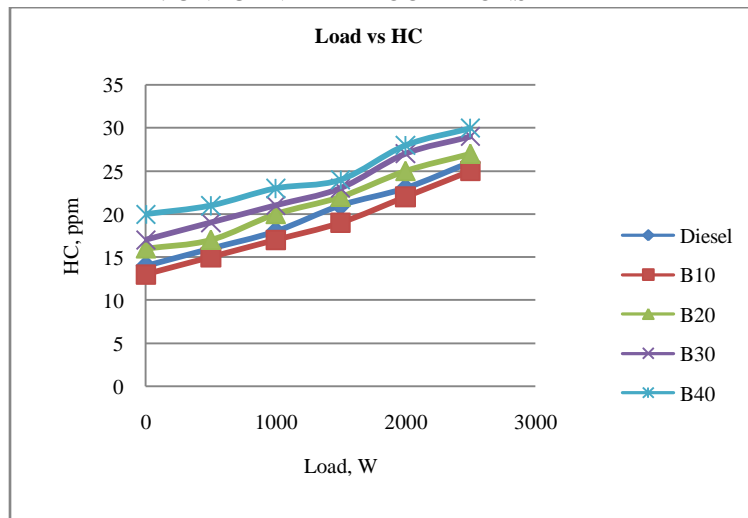
Load Vs Hydro carbons
