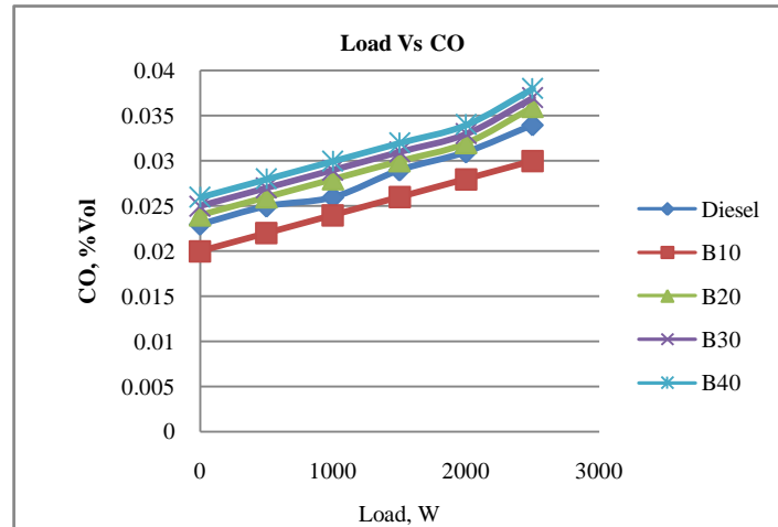
Load Vs Carbon monoxide
