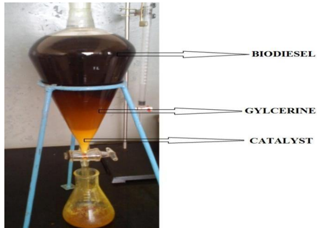
Separating funnel
