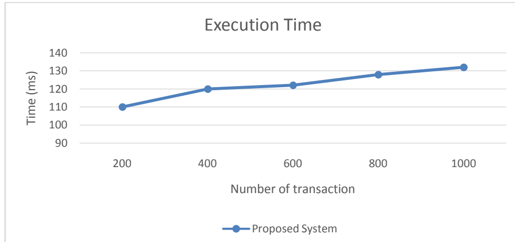
Figure 3: Execution Time vs. Number of Records
