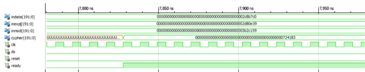
RSA decryption
