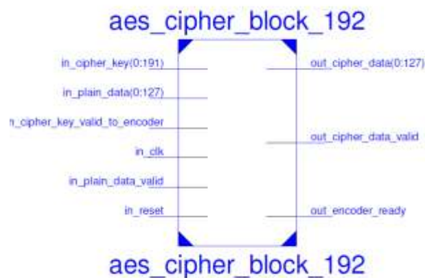
AES rtl
