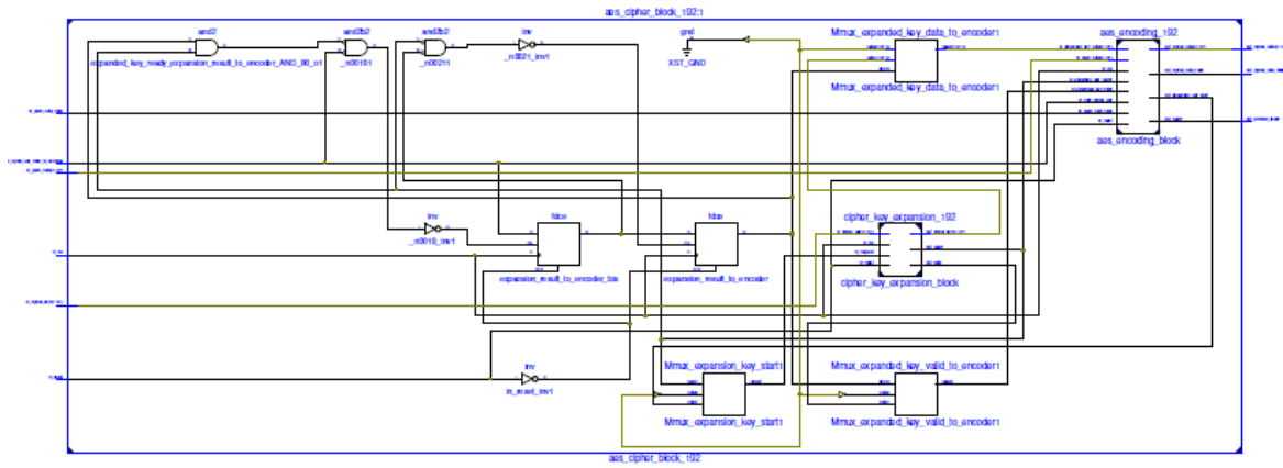
AES rtl
