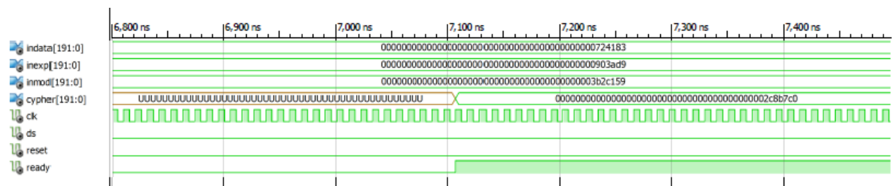
RSA encryption
