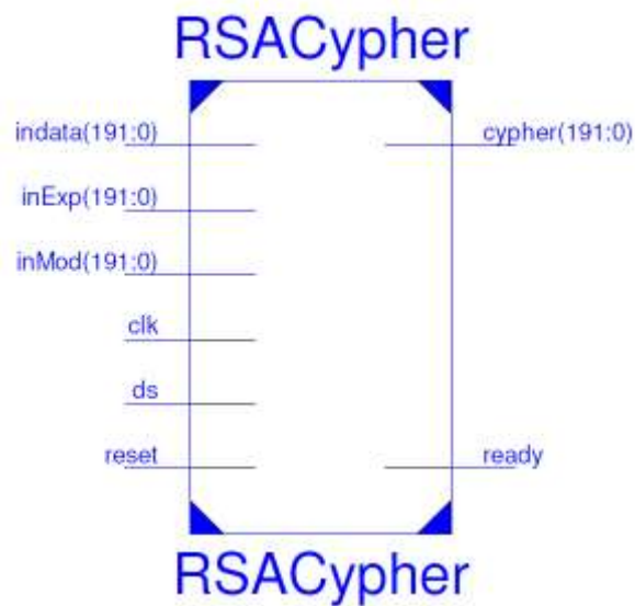
RSA rtl
