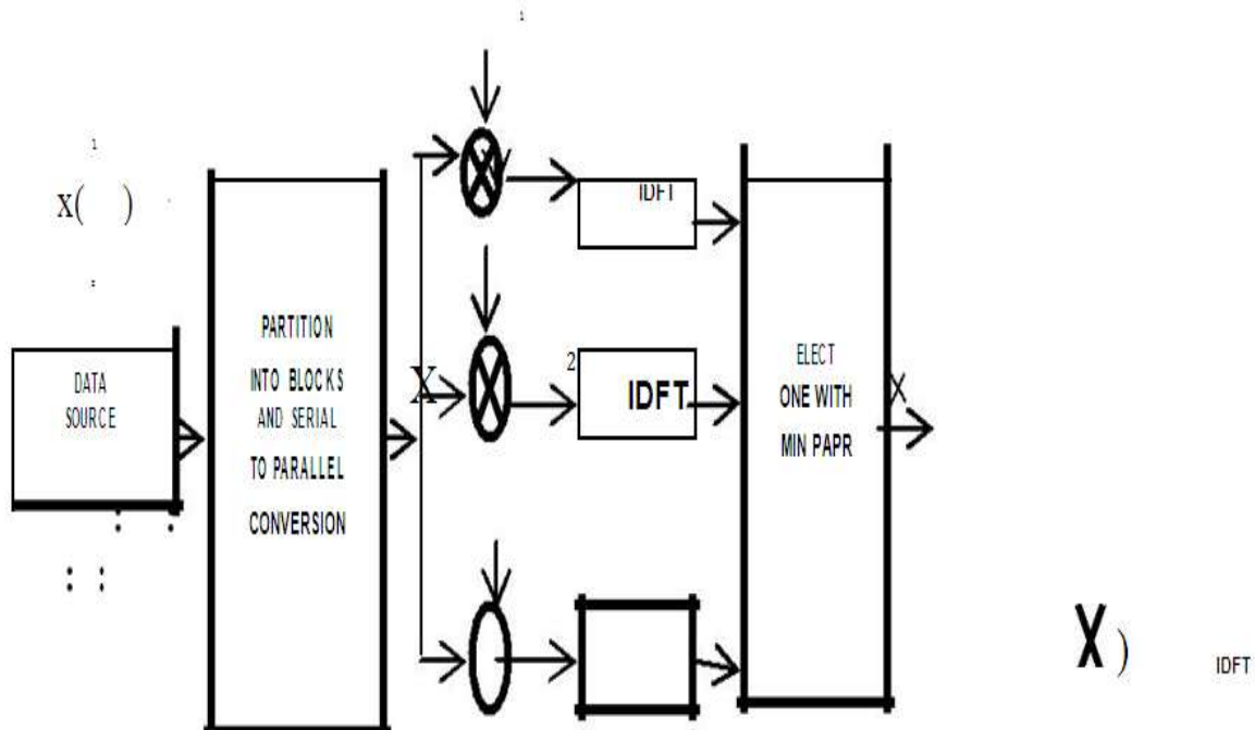
Figure 2: The Block Diagram of Selected Mapping Technique [12]
