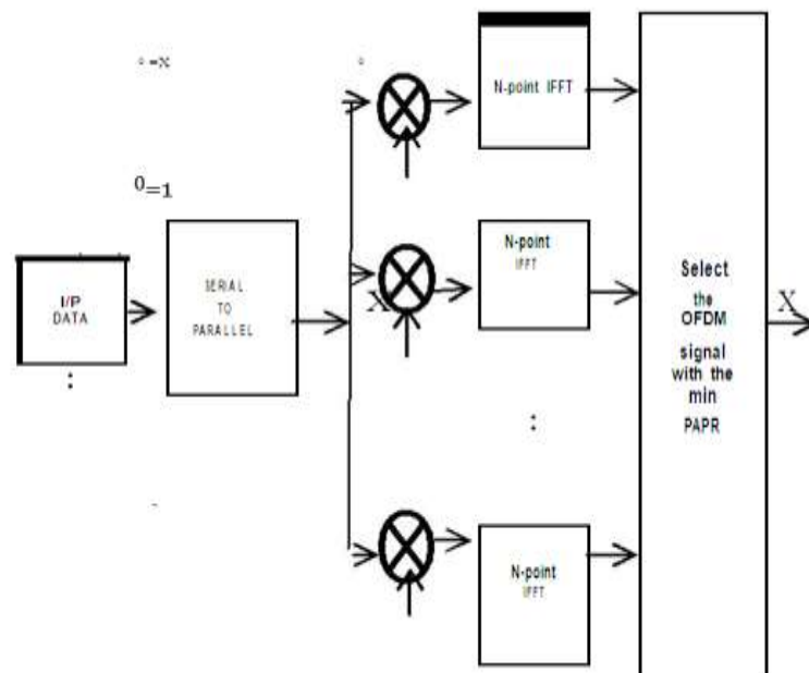
Figure 4: Block Diagram Of OFDM transmitter with SLM Technique [12]
