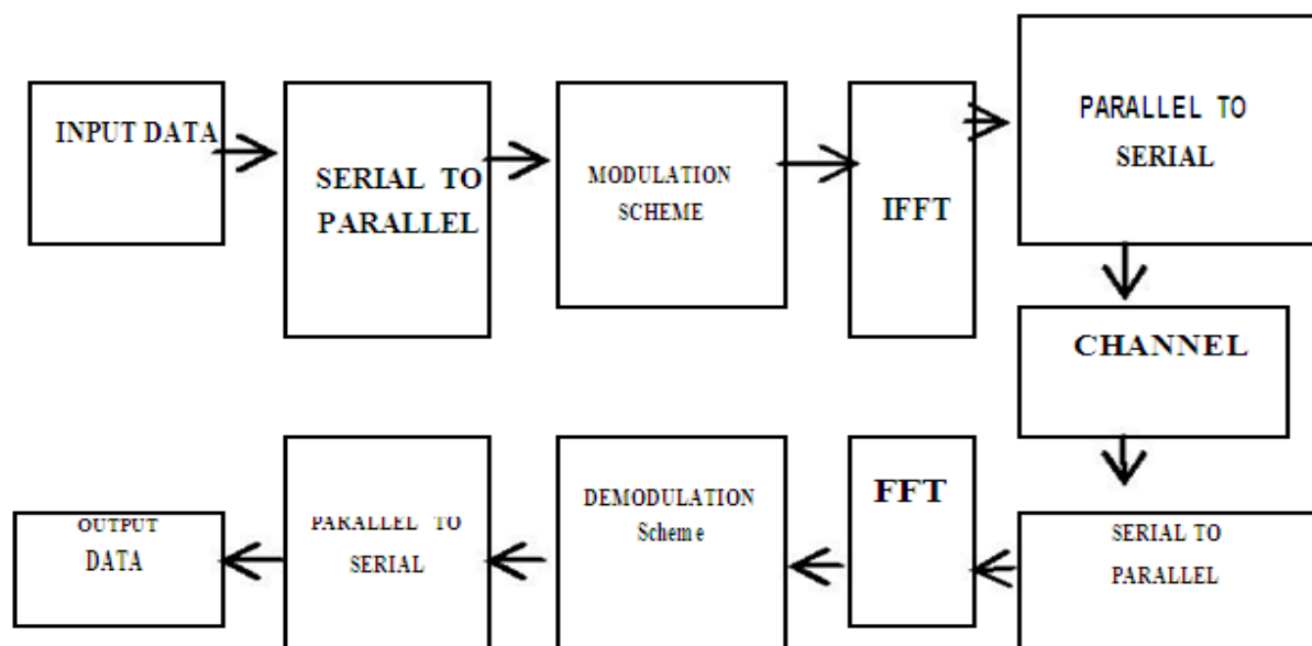
Figure 1: Block diagram of an OFDM system [13]
