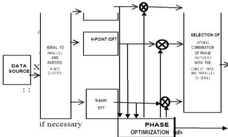
Figure 3: Block diagram of PTS technique for PAPR reduction [3]
