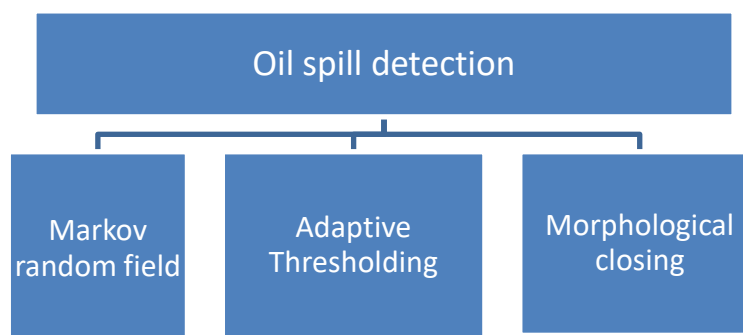
Figure2. Methodology
