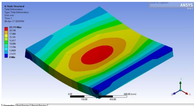
Figure 7. Bubble_Slab_64_100 Deformation
