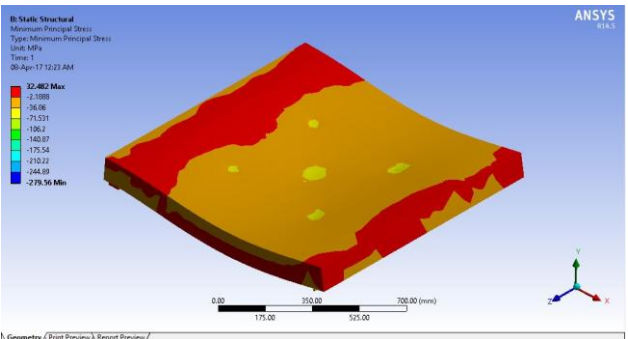
Figure 10. Bubble_Slab_80_100 Stress
