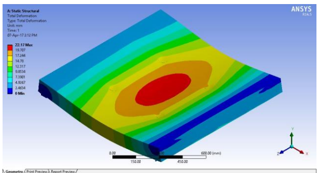
Figure 9. Bubble_Slab_80_100 Deformation
