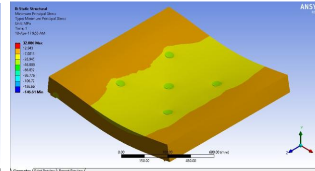
Figure 16. Bubble_Slab_64_125 Stress
