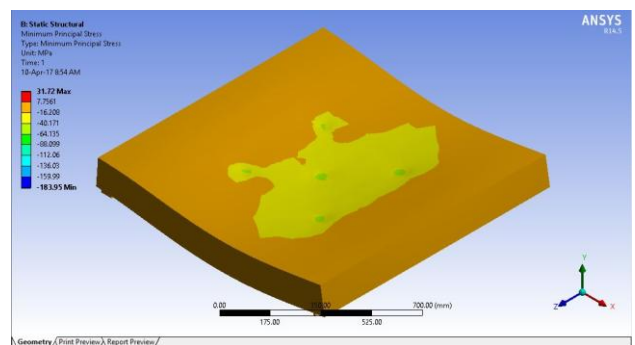
Figure 18. Bubble_Slab_100_125 Stress
