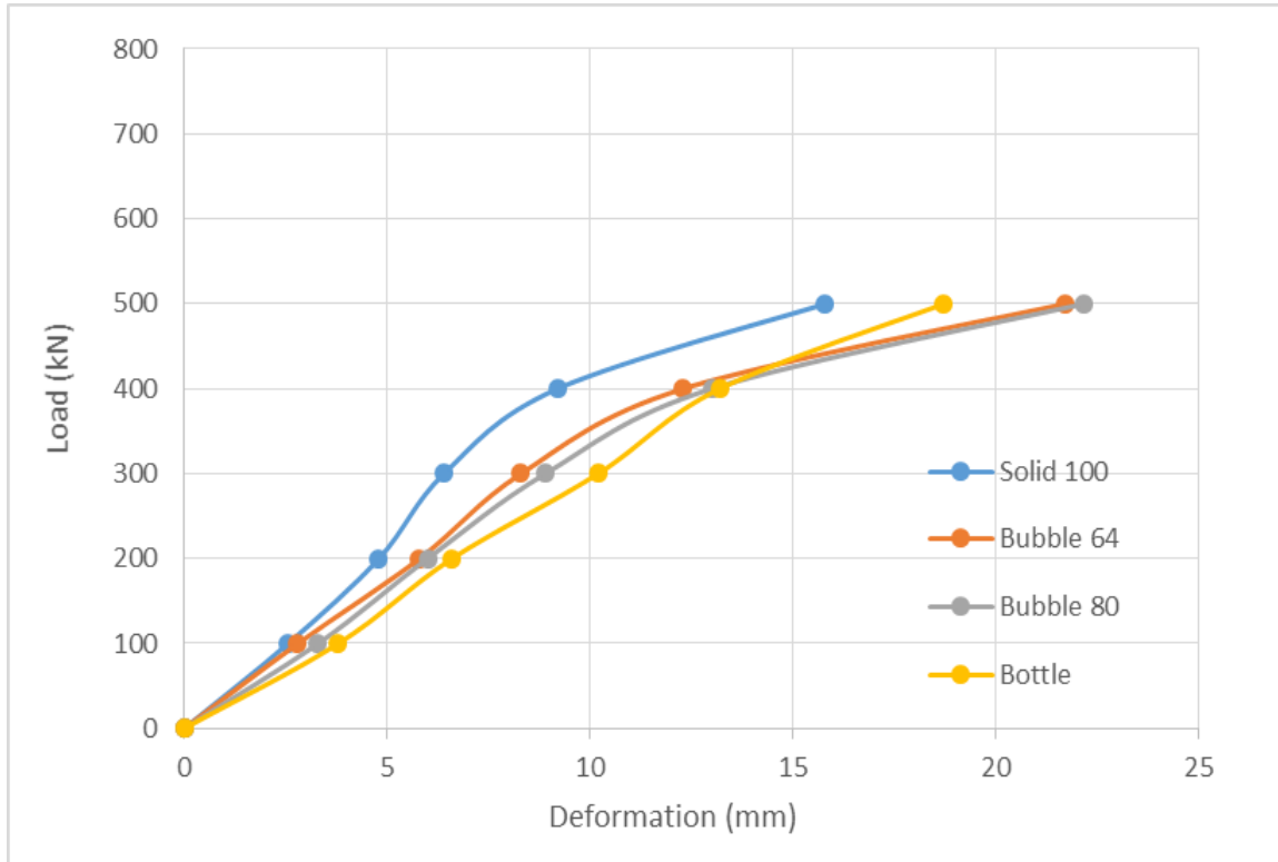
Figure 20. Load versus Deformation Relationship (H=100mm)
