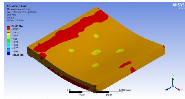
Figure 14. Bottle_Slab_50/162_100 Stress
