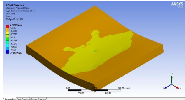
Figure 6. Solid_Slab_100 Stress
