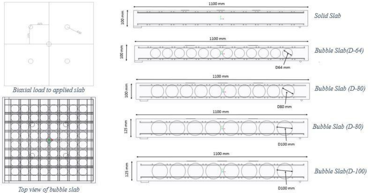
Figure 3. Cross-Section of the slab model
