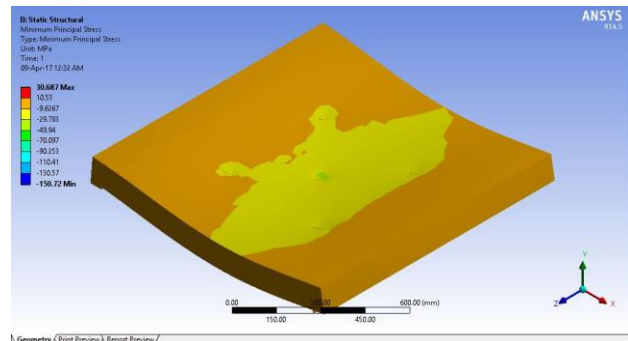
Figure 8. Bubble_Slab_64_100 Stress
