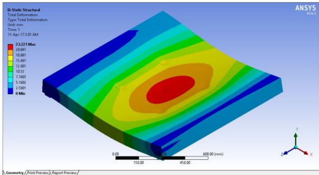
Figure 11. Bottle_Slab_50/162_100 Deformation
