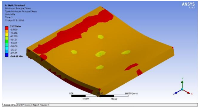
Figure 12. Bottle_Slab_50/162_100 Stress
