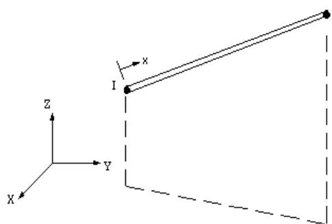
Figure 2. LINK8 Geometry
