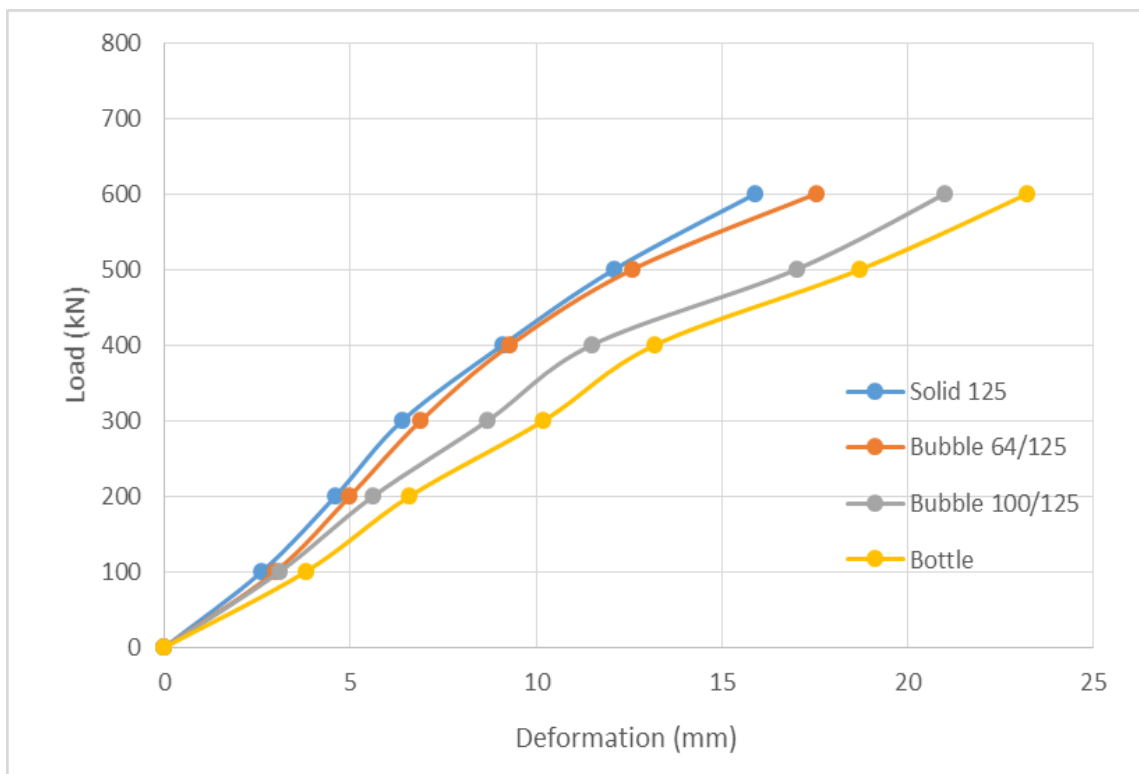
Figure 21. Load versus Deformation Relationship (H=125mm)
