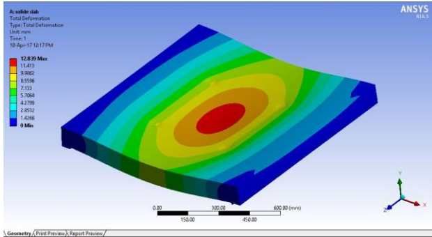
Figure 5. Solid_Slab_100 Deformation
