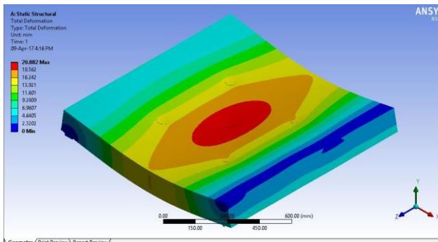
Figure 15. Bubble_Slab_64_125 Deformation
