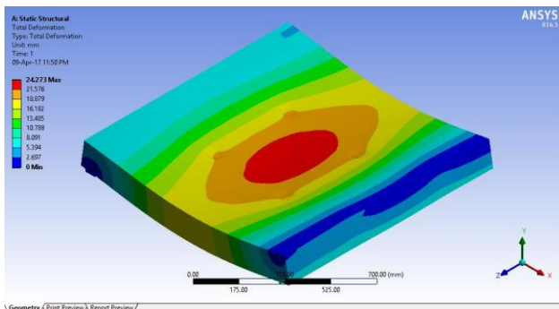
Figure 17. Bubble_Slab_100_125 Deformation
