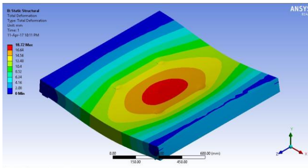
Figure 13. Bottle_Slab_50/162_100 Deformation
