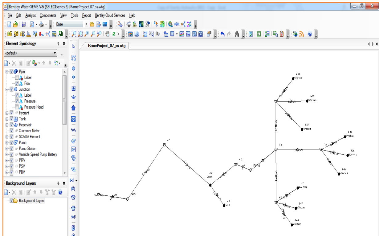
FIGURE 2. WATERGEMS MODEL
