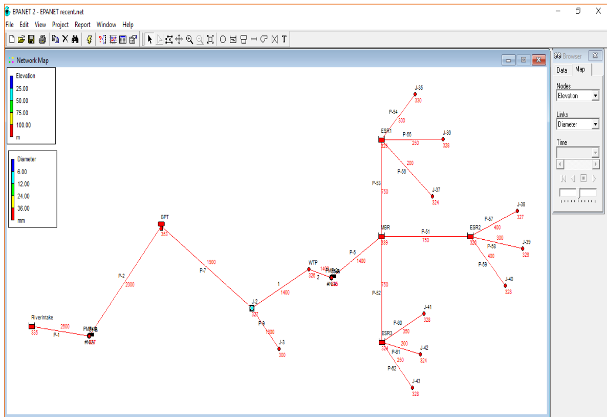
Figure 3. EPANET model
