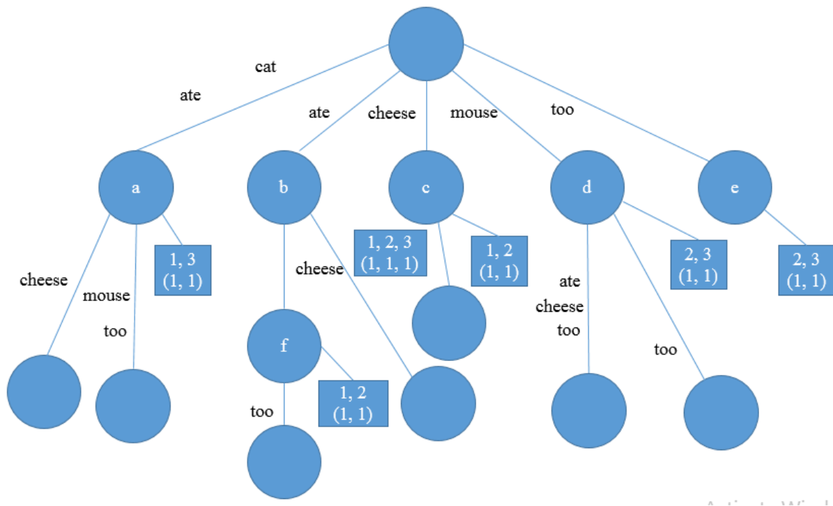
Fig. 1. The suffix tree of tree documents “cat ate cheese,” “mouse ate cheese too,” and “cat ate mouse too.”
