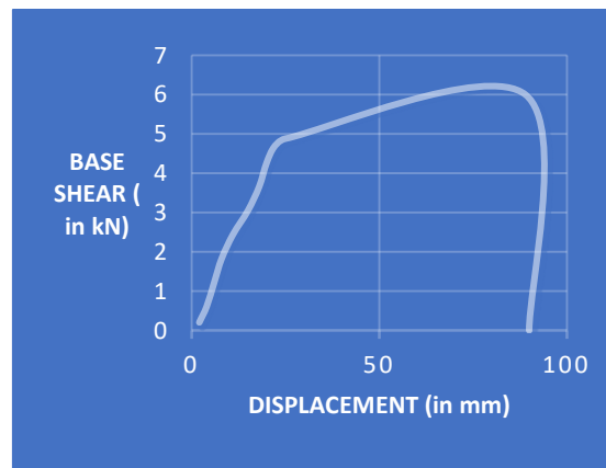
PUSHOVER CURVE FOR SHAFT STAGING
