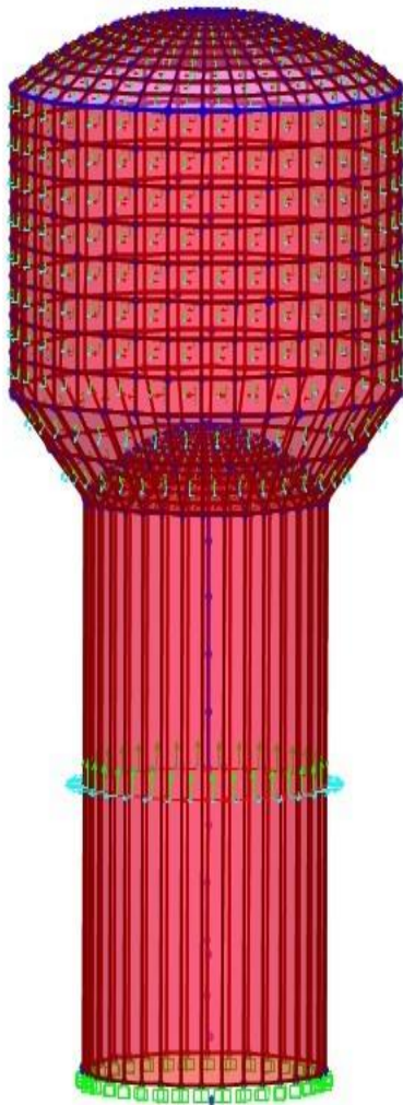
SAP 2000 MODEL FOR INTZE TANK WITH SHAFT STAGING
