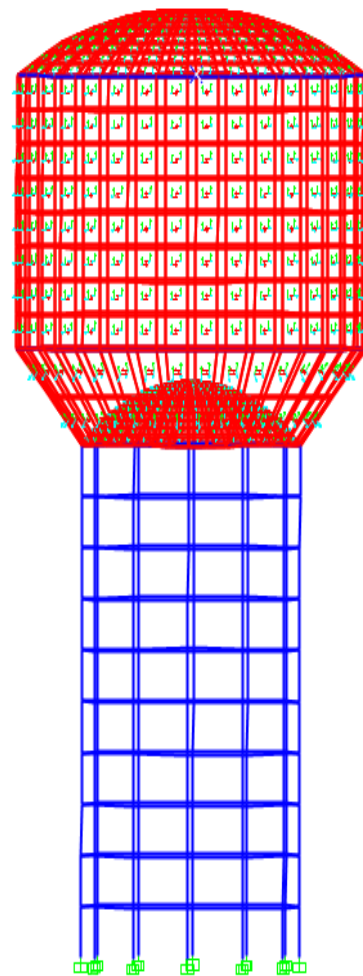
SAP 2000 MODEL FOR INTZE TANK WITH FRAME STAGING
