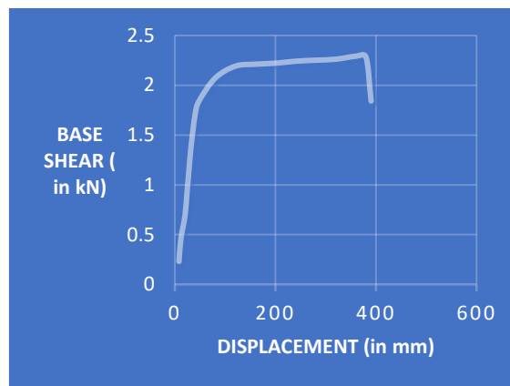
PUSH OVER CURVE FOR FRAME STAGING
