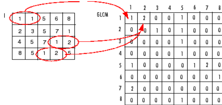
Figure 4: Gray-level co-occurrence matrix
