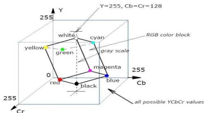
Figure 3: YCbCr Color Space
