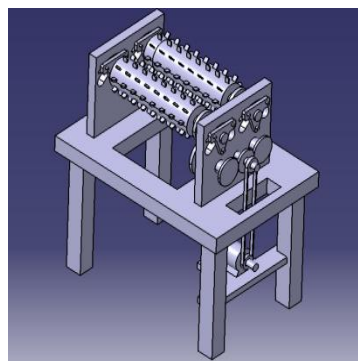
Fig 2 - Cad Model of Coconut Dehusking Machine
