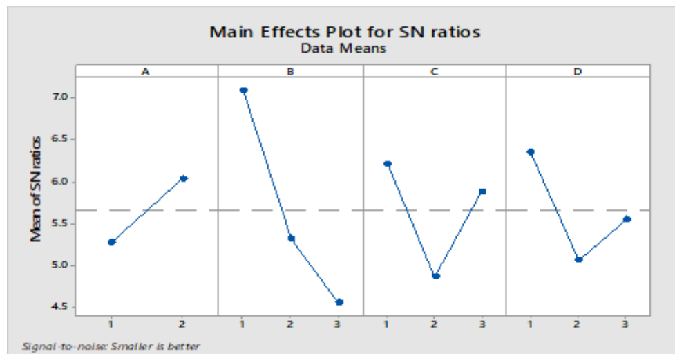
Figure 2 Main Effect plot for Surface Roughness
