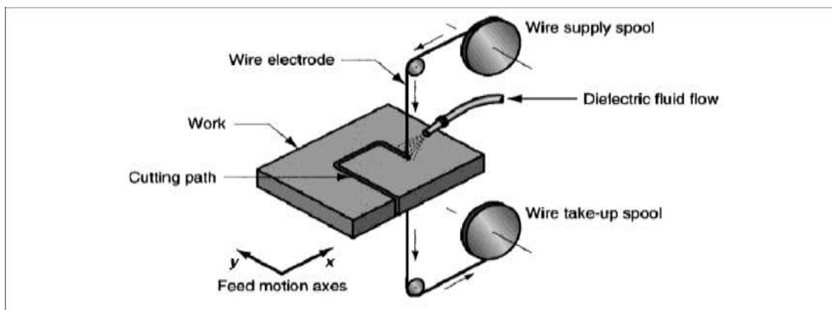
Figure 1 Wire EDM process
