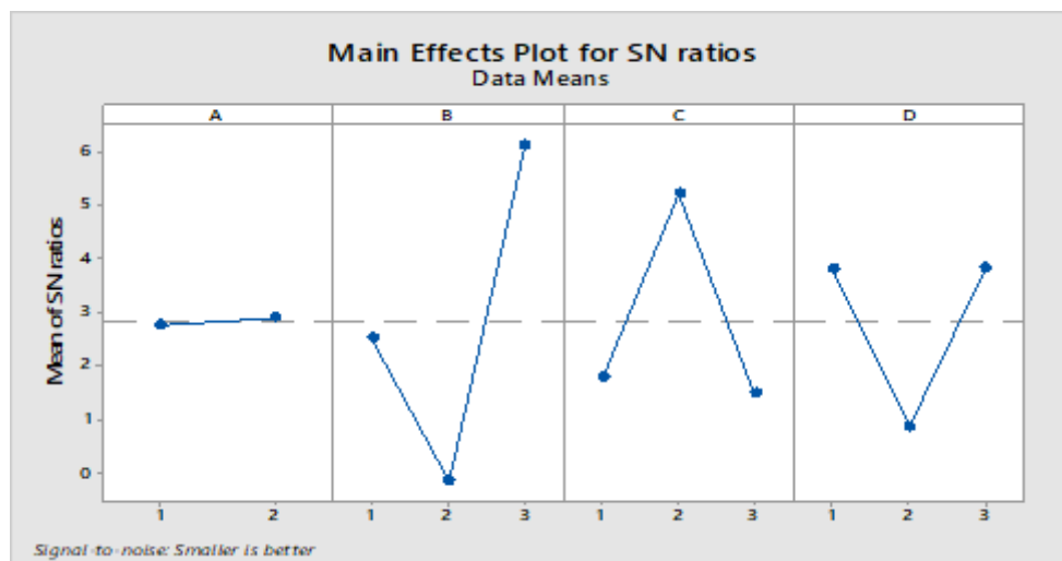
Figure 3 Main Effect Plot for Dimension Deviation
