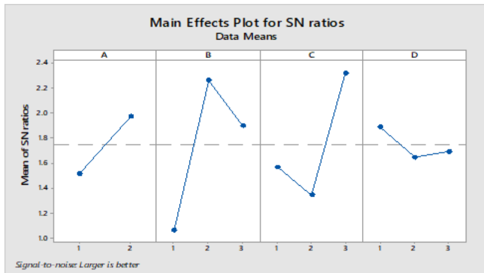
Figure 4 Main Effect Plot for Material Removal Rate
