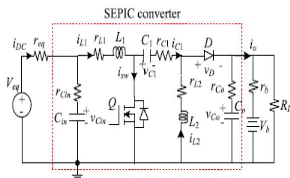
Fig.3.1.SEPIC Converter.
