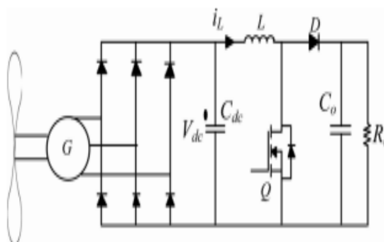
Fig.2.1. WECS Configuration.
