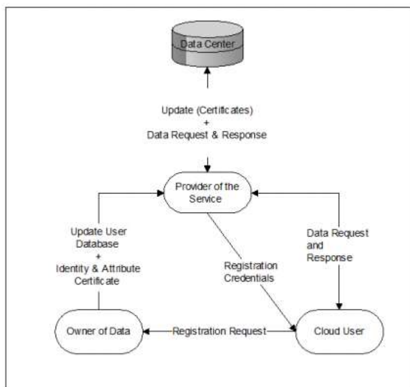
Figure 4. User Registration
