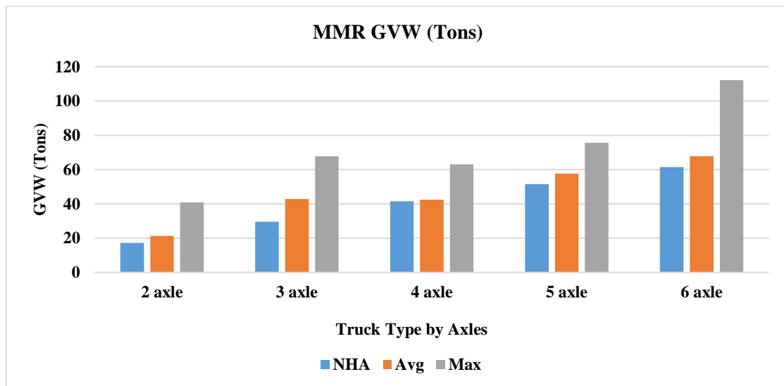
Figure 2 MMR GVW
