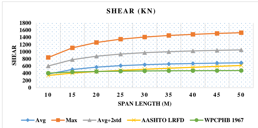
Figure 6 Shears
