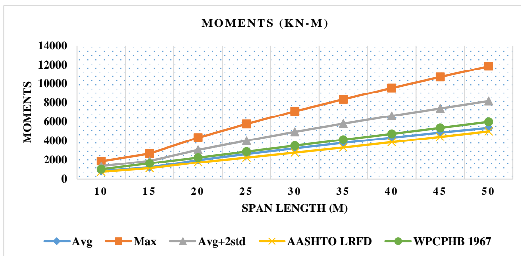
Figure 5 Moments
