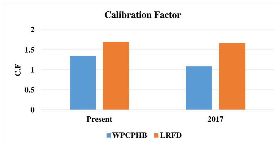
Figure 8 C.F comparison
