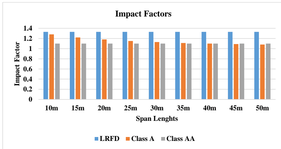
Figure 4 Impact Factors
