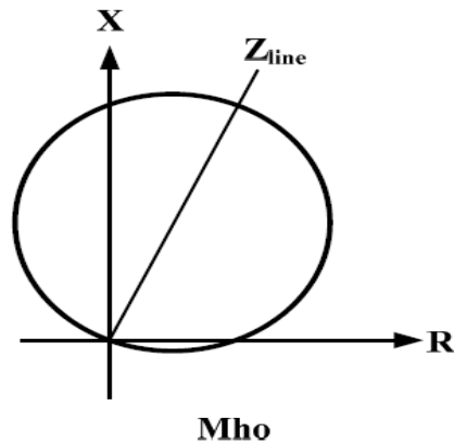
Figure 1.Mho Relay Characteristics [12]
