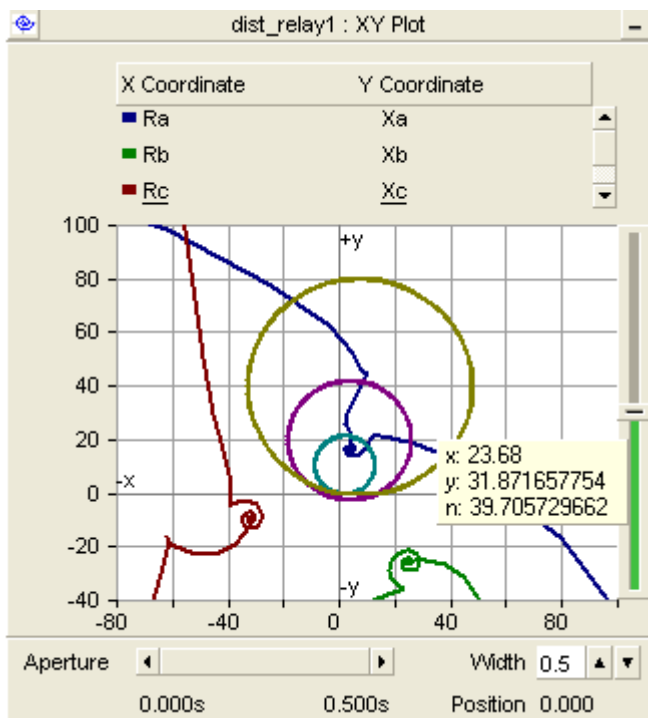
Figure 8 Line-Ground Fault
