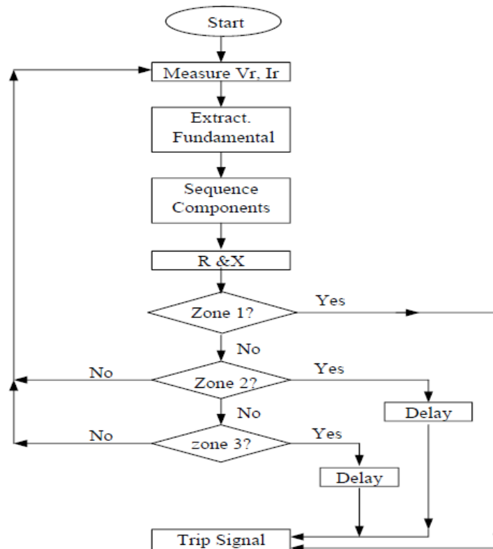
Figure 3. Algorithm for the Mho Relay Protection [1]
