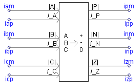
Figure 5.Input to the sequence component Block in PSCAD
