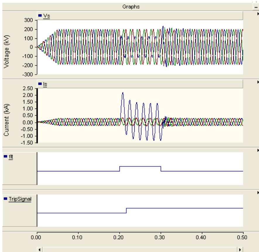
Figure 7 Waveform for the distance protection
