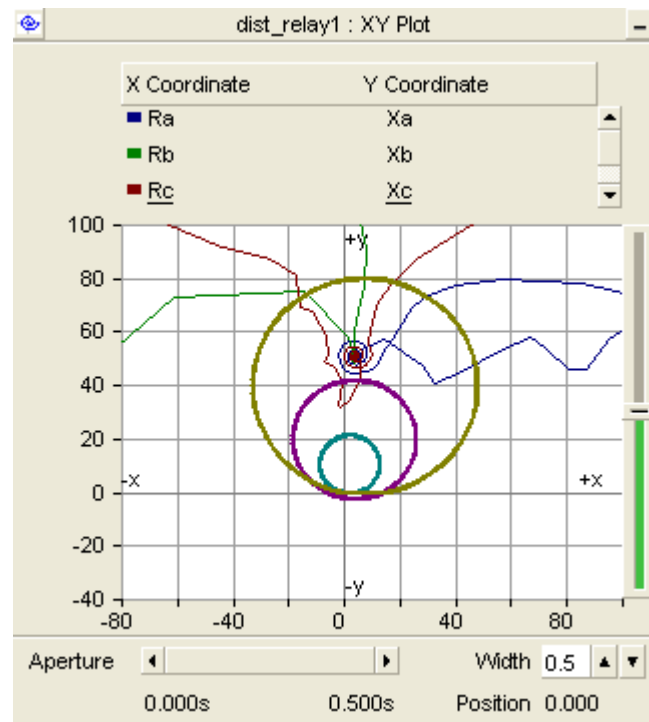
Figure 10 L-L-L Fault
