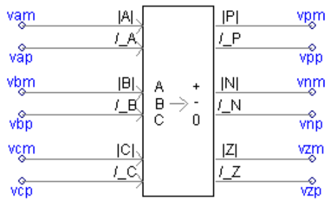
Figure 5.Input to the sequence component Block in PSCAD
