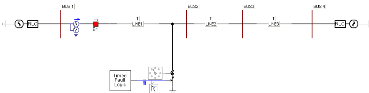
Figure 6 Systems Modelling of Transmission Line in PSCAD
