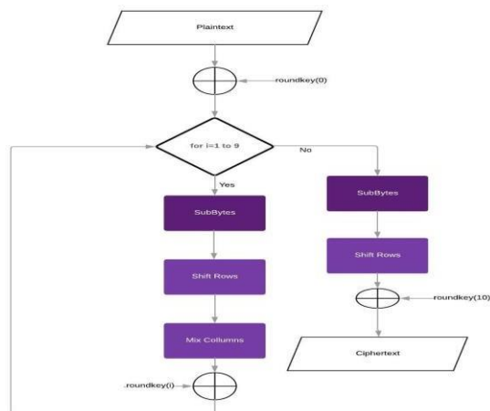
Fig. 3. Flowchart of AES encryption method.
