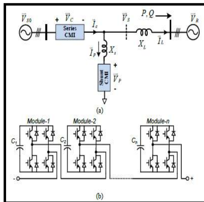
Figure 5.2 New transformer-less UFPC, (a) System Configuration of Transformer-less UPFC , (b) One phase of the cascaded multilevel inverter
