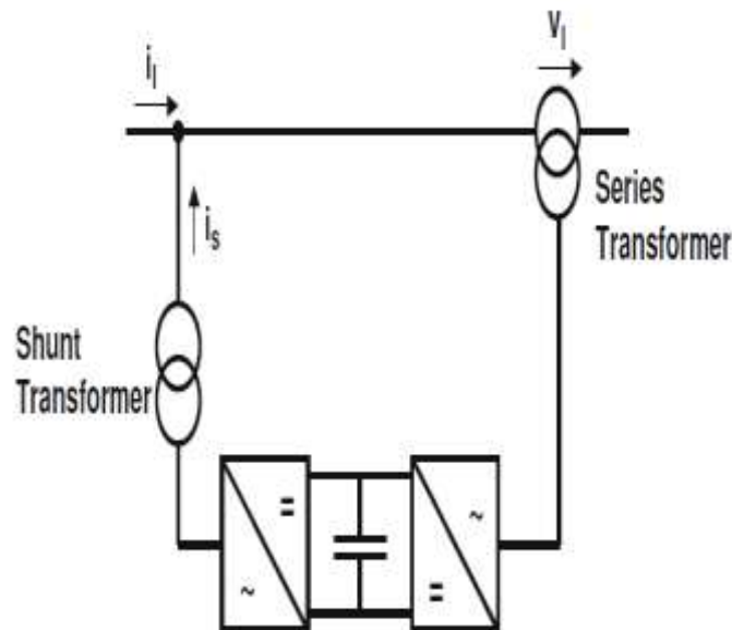
Figure 4.1 Principle configuration of an UPFC
