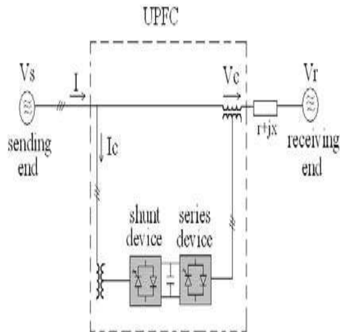
Figure 4.2 UPFC Set up Scheme
