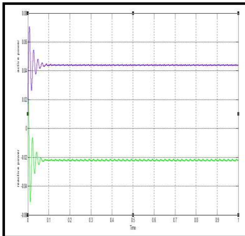
Figure 6.10 Active and Reactive Power at Source Side
