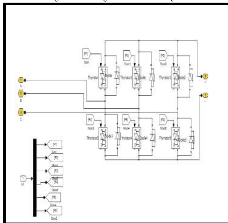
Figure 6.4 VSC configuration in UPFC design
