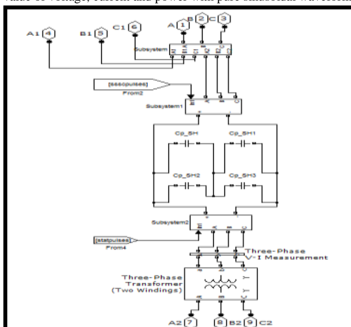
Figure 6.6 Controlling Subsystem
