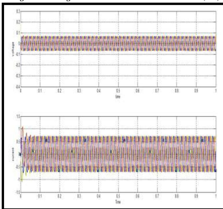
Figure 6.8 Voltage and Current waveform at Load Side
