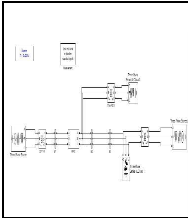
Figure 6.1 Three phase compensated network connect with UPFC system
