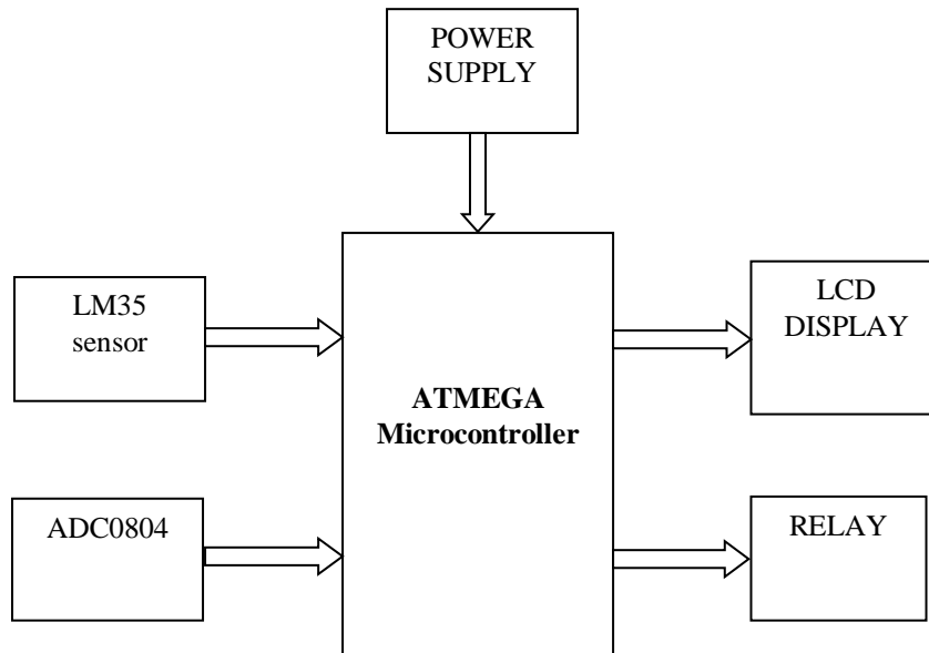
Fig 2. Block diagram of underground fault system
