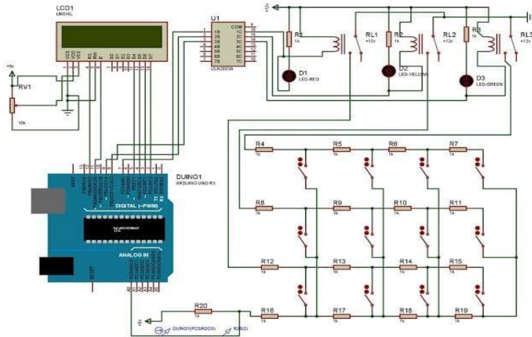
Fig 1 Resistor and Switches Connection
