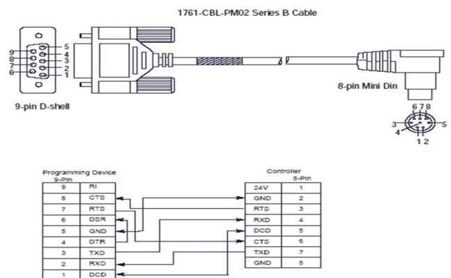
Fig.12 Embedded Serial Port Wiring
