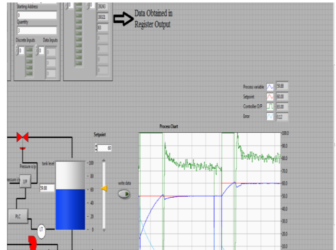
Fig.11 Developed front panel diagram
