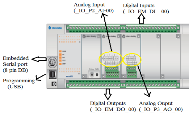
Fig.13 Allen Bradley PLC
