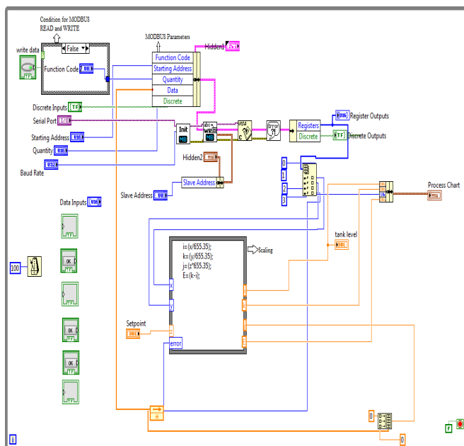
Fig.10 Developed block diagram for MODBUS Read and Write
