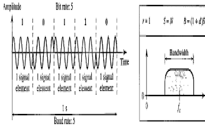
Figure 1. Binary phase shift keying.[14]
