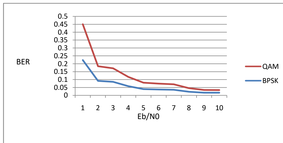
Figure 4. BER of QAM BPSK modulation in Rayleigh Fading channel using BCH encoding.
