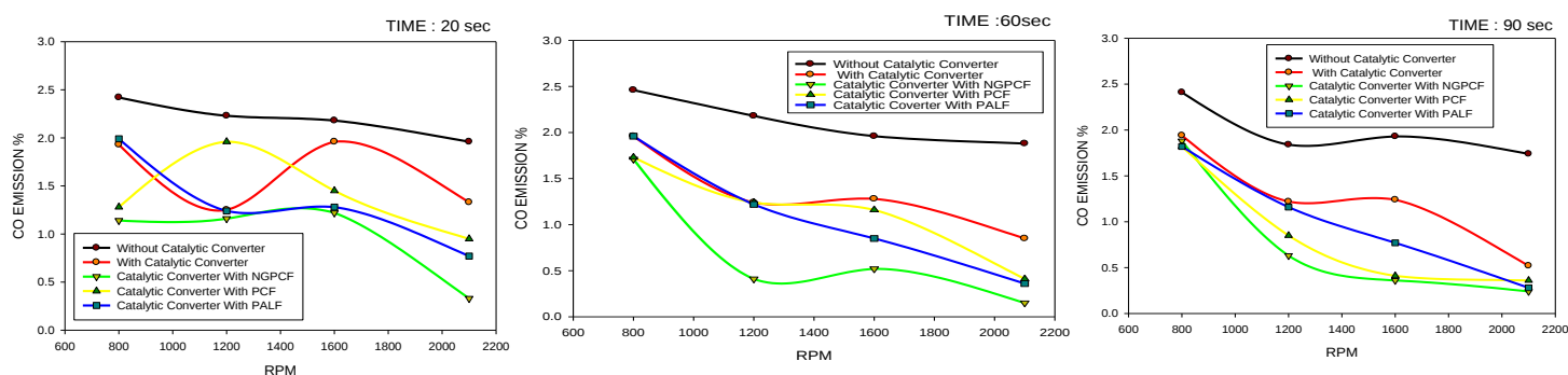
Figure 12. Graph for value of CO At different TIME, RPM for different Pre-filter.
