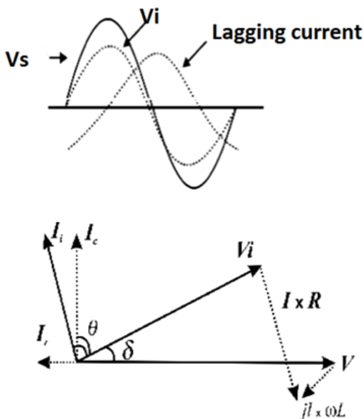
Fig.3.1(b): The Inductive mode V_s > V_i
