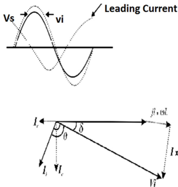
Fig.3.1(c): The Capacitive mode V_s < V_i
