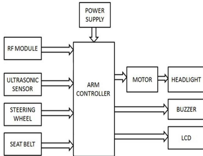
Figure 1. Block diagram of vehicle safety and automotive driver assistance system.
