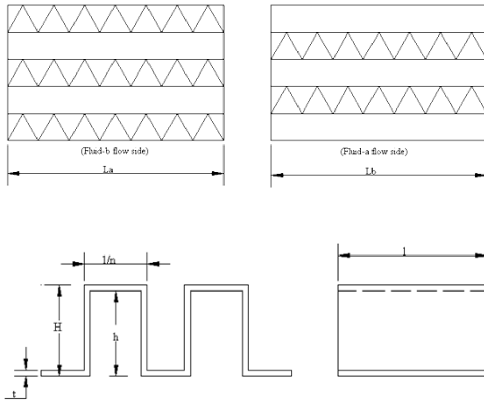
Figure 1: Front view and side view of plate-fin heat exchanger and offset-strip fin.
