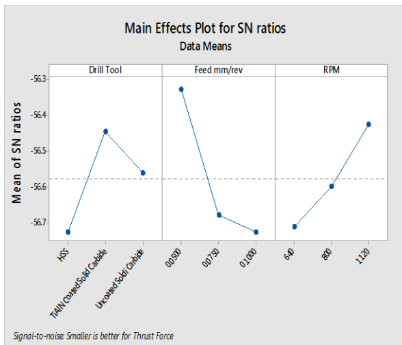
Figure-4 Main effect plot for S/N ratio for Thrust Force
