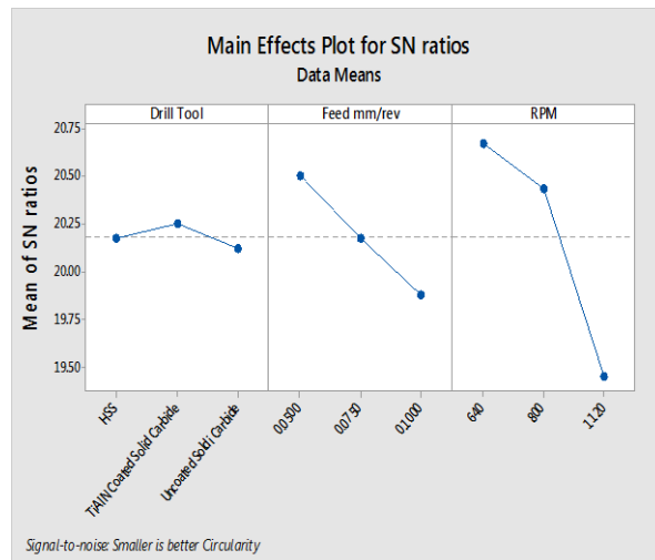
Figure-5 Main effect plot for S/N ratio for Circularity
