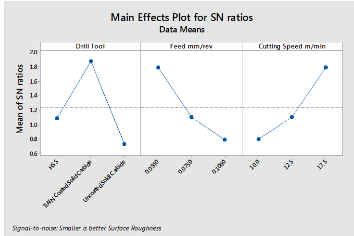
Figure-6 Main effect plot for S/N ratio for Surface Roughness
