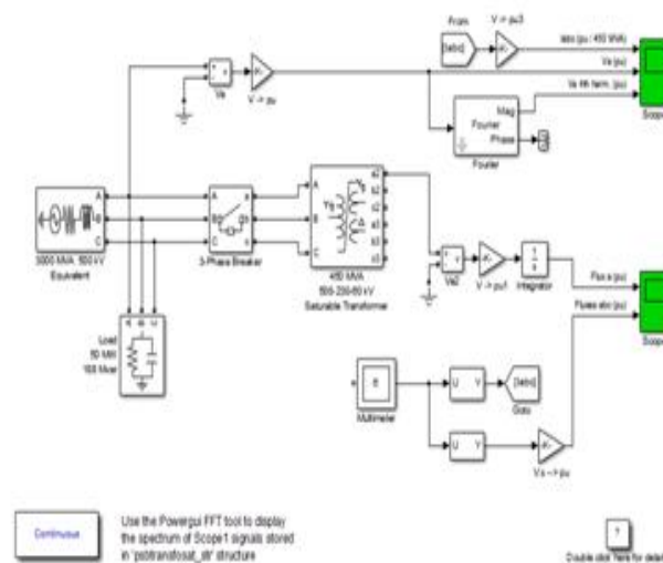
Figure 1: MATLAB-SIMULINK model to establish the fuzzy control algorithm.
