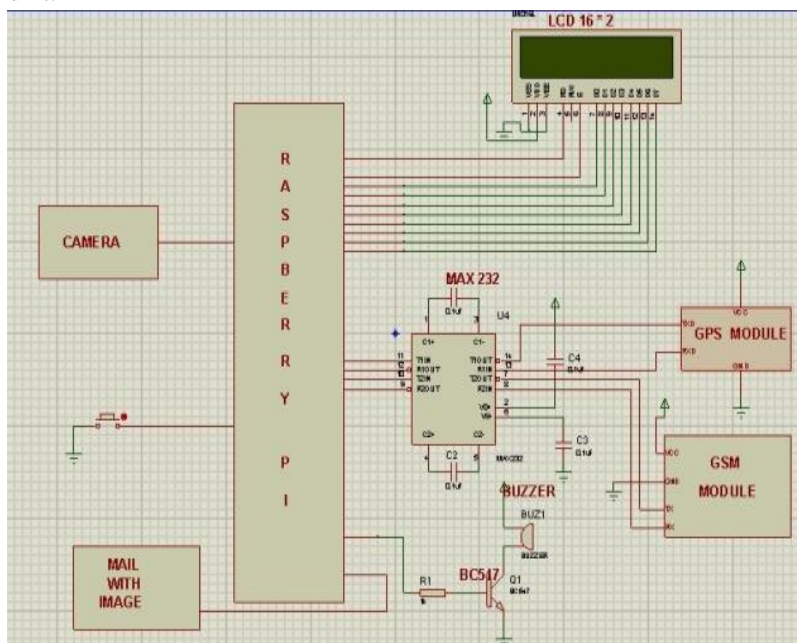
Fig. 2 Circuit diagram
