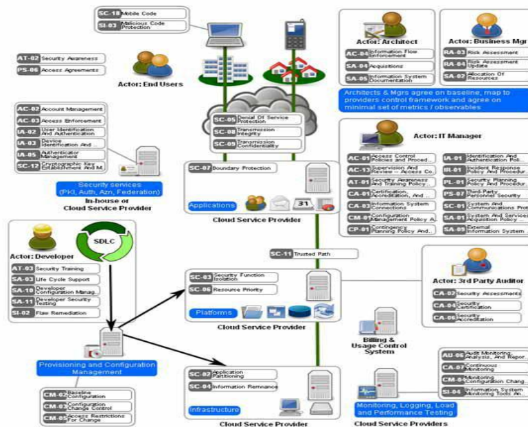
Figure 1. Cloud Computing Model - Open Secure Architecture [OSA09].
