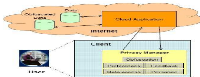
Figure 3 Overview of Privacy Manager.
