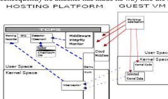
Figure 4 TCPS Architecture.
