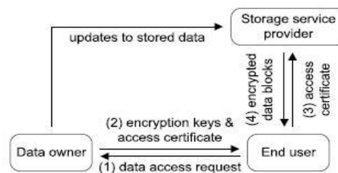
Figure 5 Illustration of application scenario
