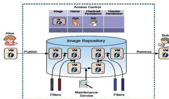
Figure 2. Architecture of Mirage Image Management System.
