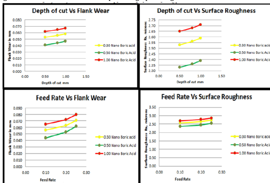
Figure-3. Behavior curve when feed rate or depth of cut kept constant
