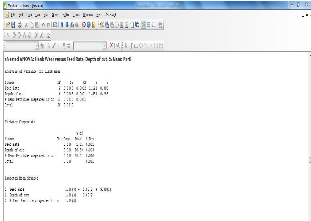
Figure-2. Analysis of Variance for Flank Wear
